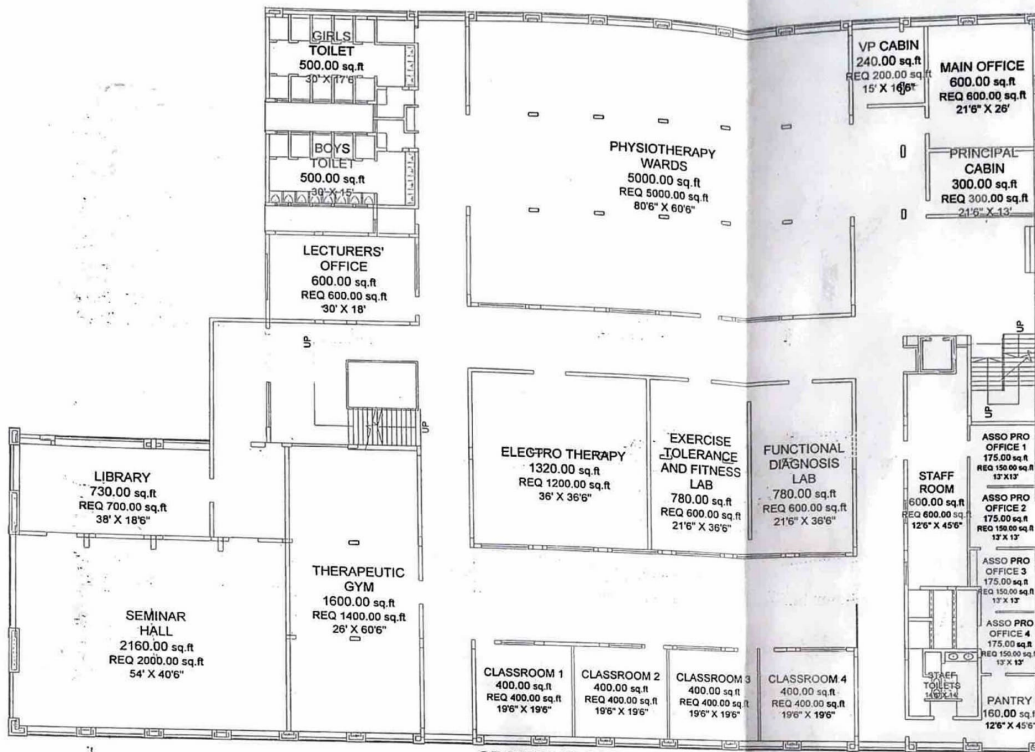
GROUND FLOOR PLAN FOR PAMILADEVI PATIL COLLEGE OF PHYSIOTHERAPY IN EXISTING EDUCATIONAL BUILDING
