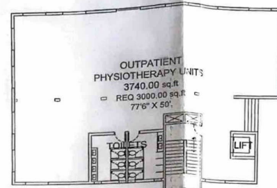
GROUND FLOOR PLAN EXISTING HOSPITAL BUILDING
